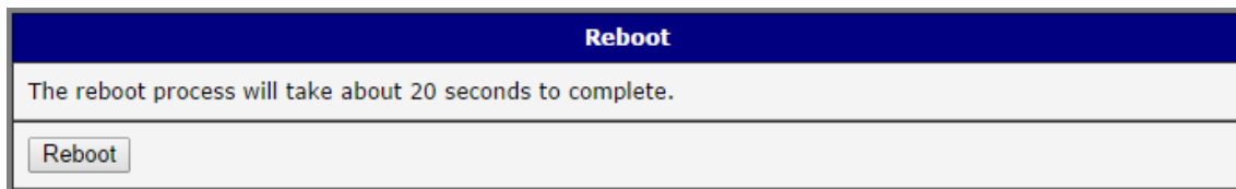
Figure 82: Reboot
