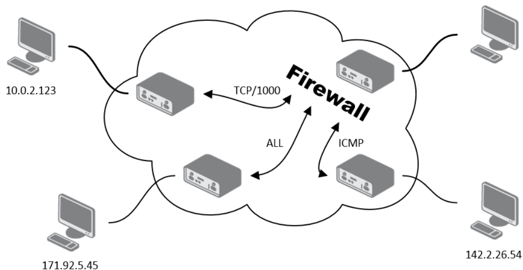
Figure 29: Topology for the Firewall Configuration Example
